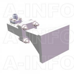
LB-42-15-C-SFSPO Standard Gain Horn Antenna 18-26.5GHz 15dB Gain SMA Female
